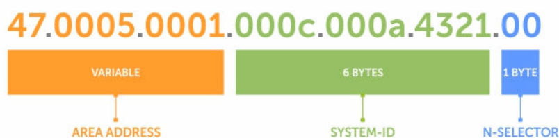
Figure 51. ISO Address Format
